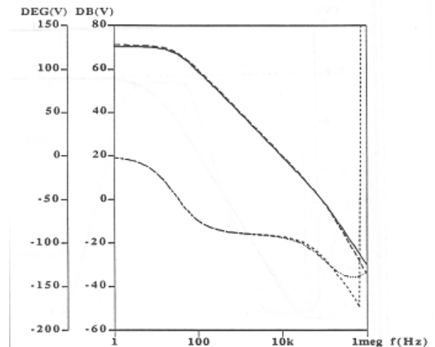
Figure 6. Frequency response curves (magnitude and phase) of the op-amp and its behavioral model.
