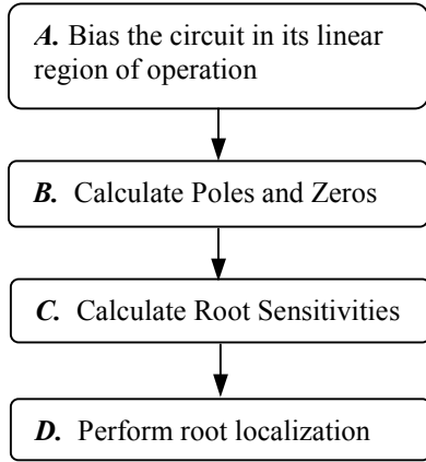
Figure 2. Analyses performed on linearized circuit.
