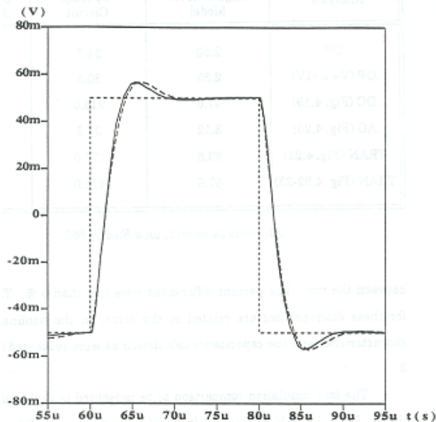
Figure 8. Small-signal transient response of the op-amp and its behavioral model in a voltage follower configuration.
