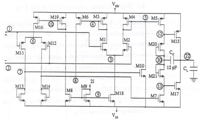
Figure 5. High Dynamic-range Op-amp
