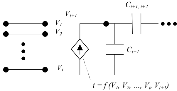
Figure 3. General representation of a physically modeled node.
