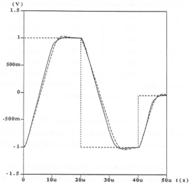
Figure 7. Large-signal transient response of the op-amp and its behavioral model in a voltage follower configuration.
