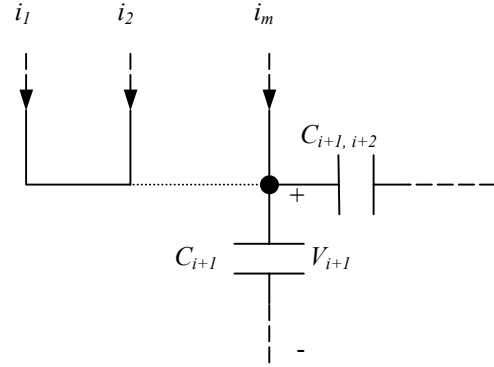
Figure 4. General node in an analog circuit.
